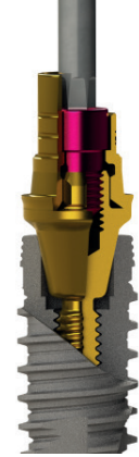
Straight Screw Channel
